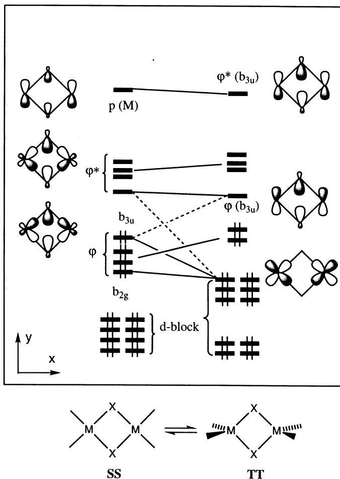
Fig. 3. Qualitative correlation diagram for the d-block and framework ( \phi and \phi^* ) orbitals of a [\text{M}_2(\mu\text{-XR}_m)_2\text{L}_4] complex in the TT and SS structures (see 3d ). The orbital occupation shown corresponds to, e.g. \text{M} = \text{Rh} , \text{XR}_m = \text{PR}_2 , and \text{L} = \text{neutral ligand} .
