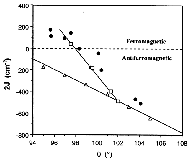
Fig. 1. Exchange coupling constant calculated for hydroxo-bridged Cu(II) complexes as a function of the Cu–O–Cu bond angle ( \theta ), with the hydrogen atom in the \text{Cu}_2\text{O}_2 plane (triangles), and with \theta optimized for different out of plane angles (white squares). The black circles represent the experimental data. Adapted from Ref. [16].
